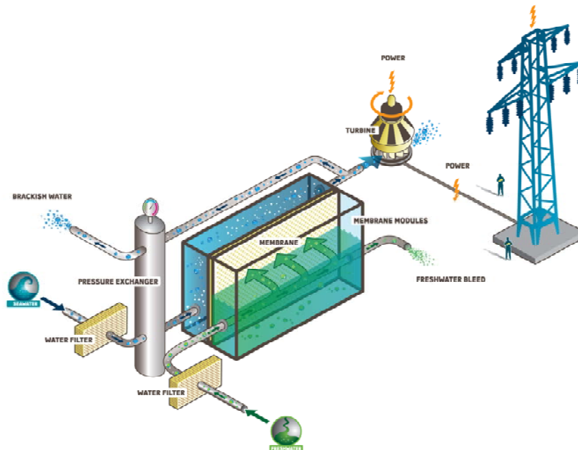
Figure 1: The principle of osmotic power is utilising the energy outcome of mixing water with different salt gradients. In the process the water with low salt gradient moves to the side with the higher salt concentration and creates increased pressure due to osmotic forces. Given the sufficient control of the pressure on the saltwater side, approximately half the theoretical energy can be transformed to electrical power, meaning that the operating pressure is in the range of 11-14 bars enabling the generation of 1MW per m 3 /s of freshwater.
