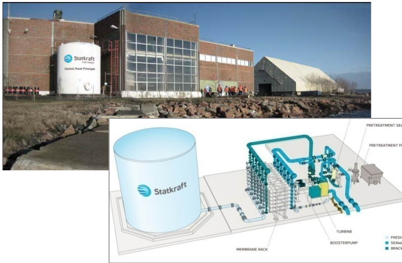
Figure 2: The prototype located at the east coast of Norway.
